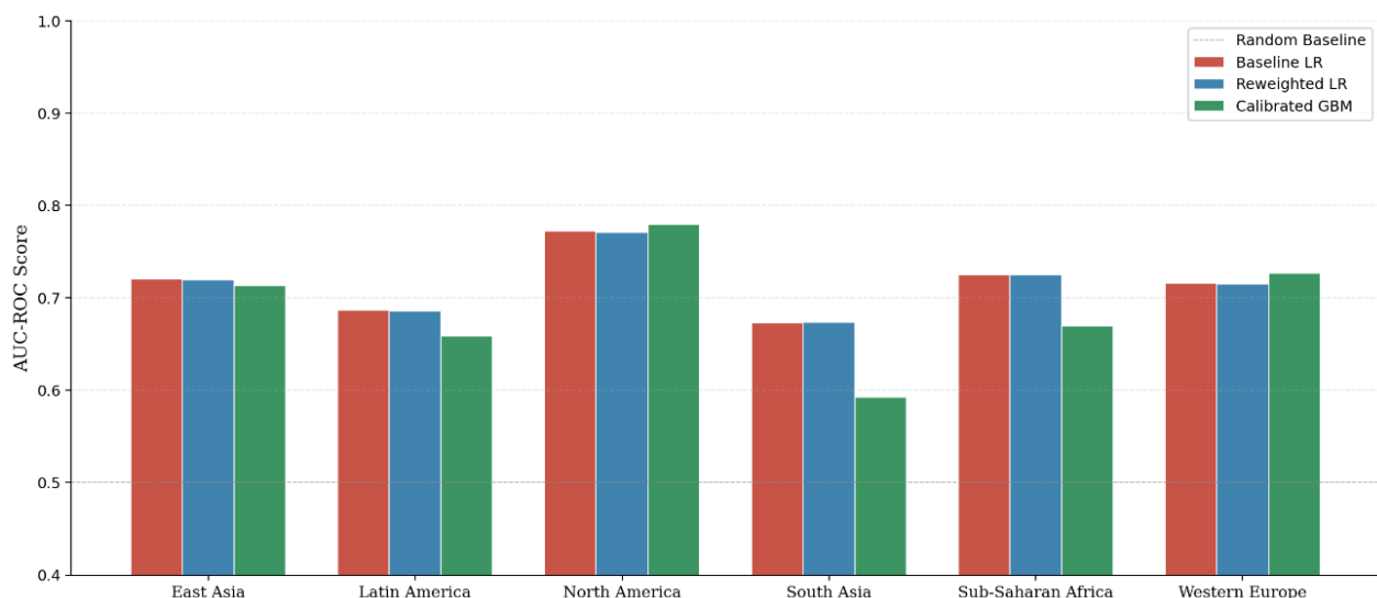
Figure 2. Cross-Regional AUC-ROC Comparison: grouped bar chart, six regions on x-axis, AUC-ROC on y-axis, three model colours
