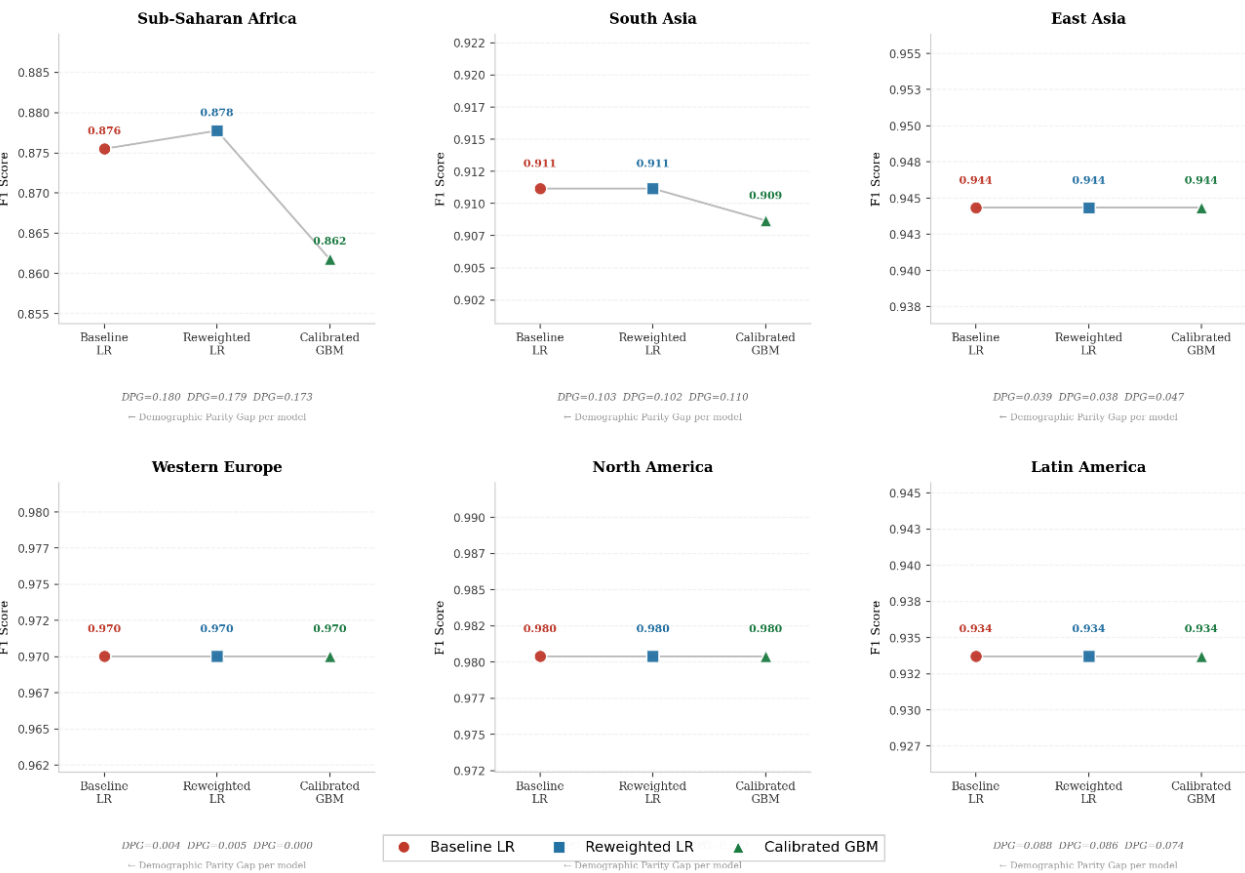
Figure 5 tracks F1 trajectories across all three model conditions for each region individually, with DPG annotated beneath each panel. Three distinct patterns emerge.
