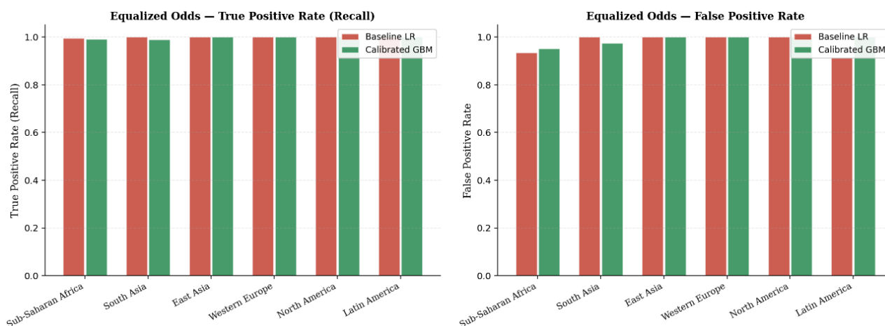
Figure 3. Equalized Odds: two-panel figure showing True Positive Rate (left) and False Positive Rate (right) per region, Baseline LR (red) vs. Calibrated GBM (green)
