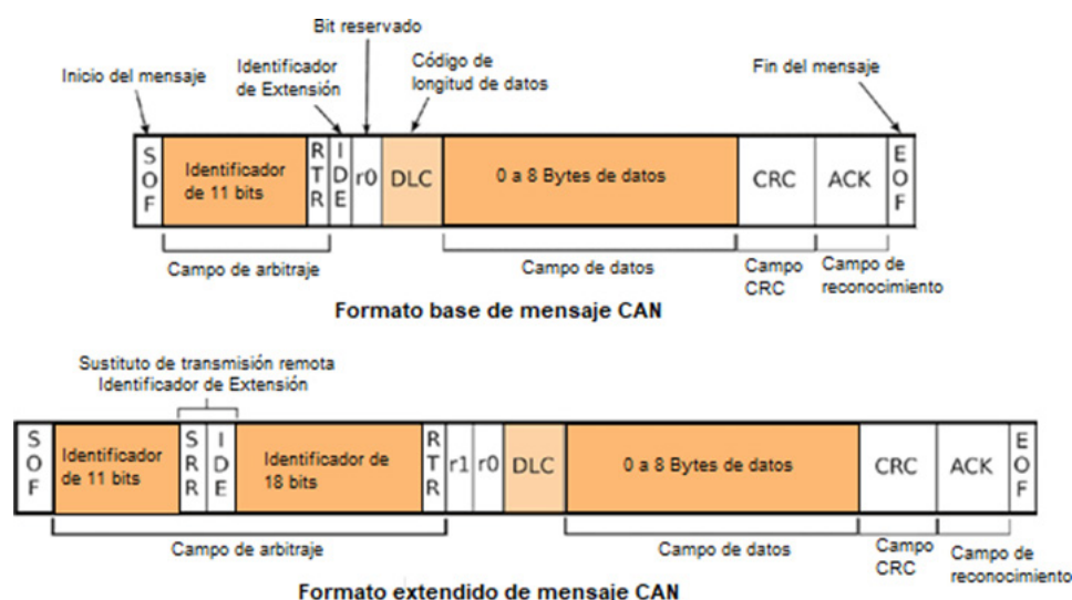
Figure 10. Message structure of the CAN communication protocol (1)
