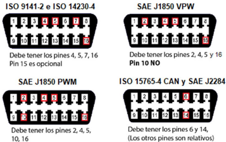
Figure 9. Connectors for OBDII protocols (23) Communication protocols
