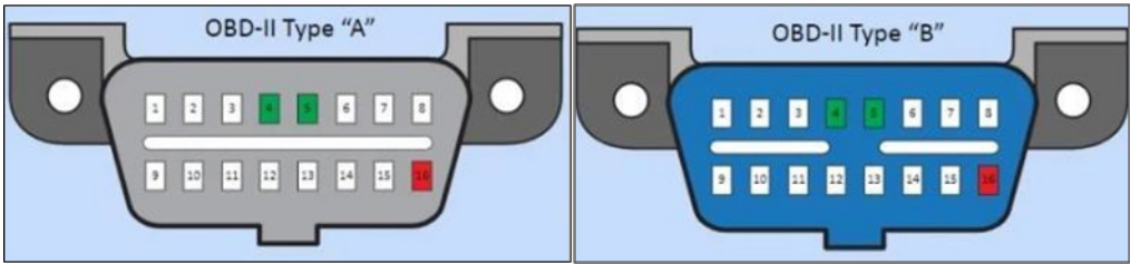
Figure 8. Interfaces for OBDII specified by SAE J1962
