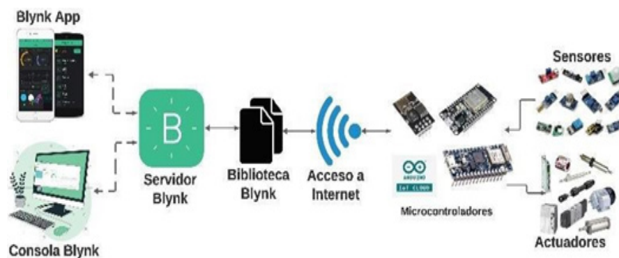
Figure 7. Integration of the Blynk platform with external devices
