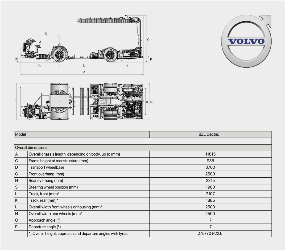
Figure 23. Volvo BZL Electric Platform
