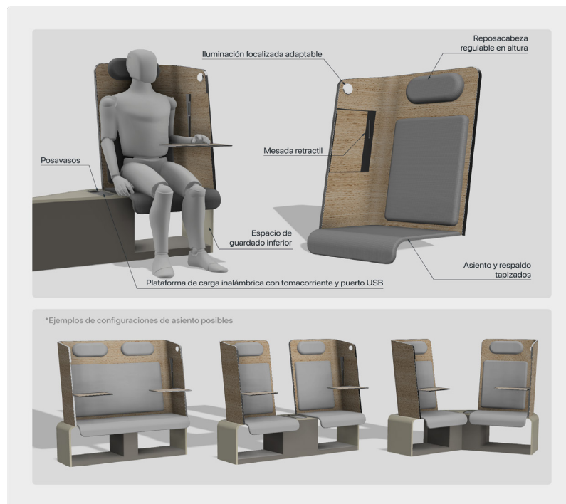
Figure 33. Detail of extended-use seats
