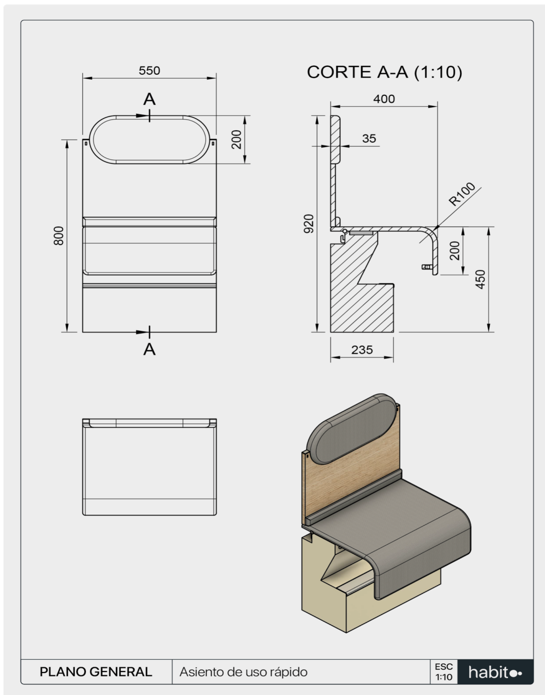
Figure 35. General plan of quick-use seat
