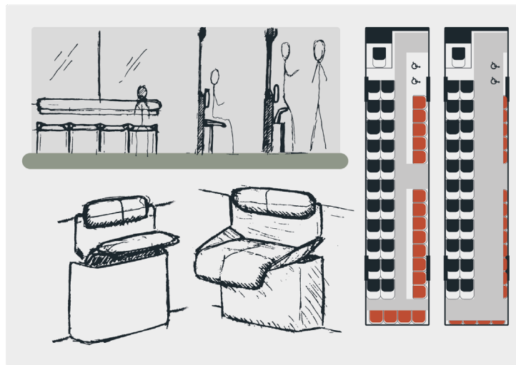
Figure 25. Design Alternatives I
