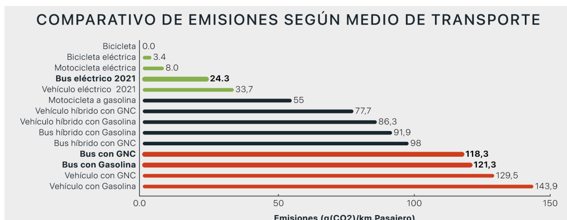
Figure 3. Comparative table of annual emissions per passenger in (g(CO 2 )/km.pasajero) for different means of transport
