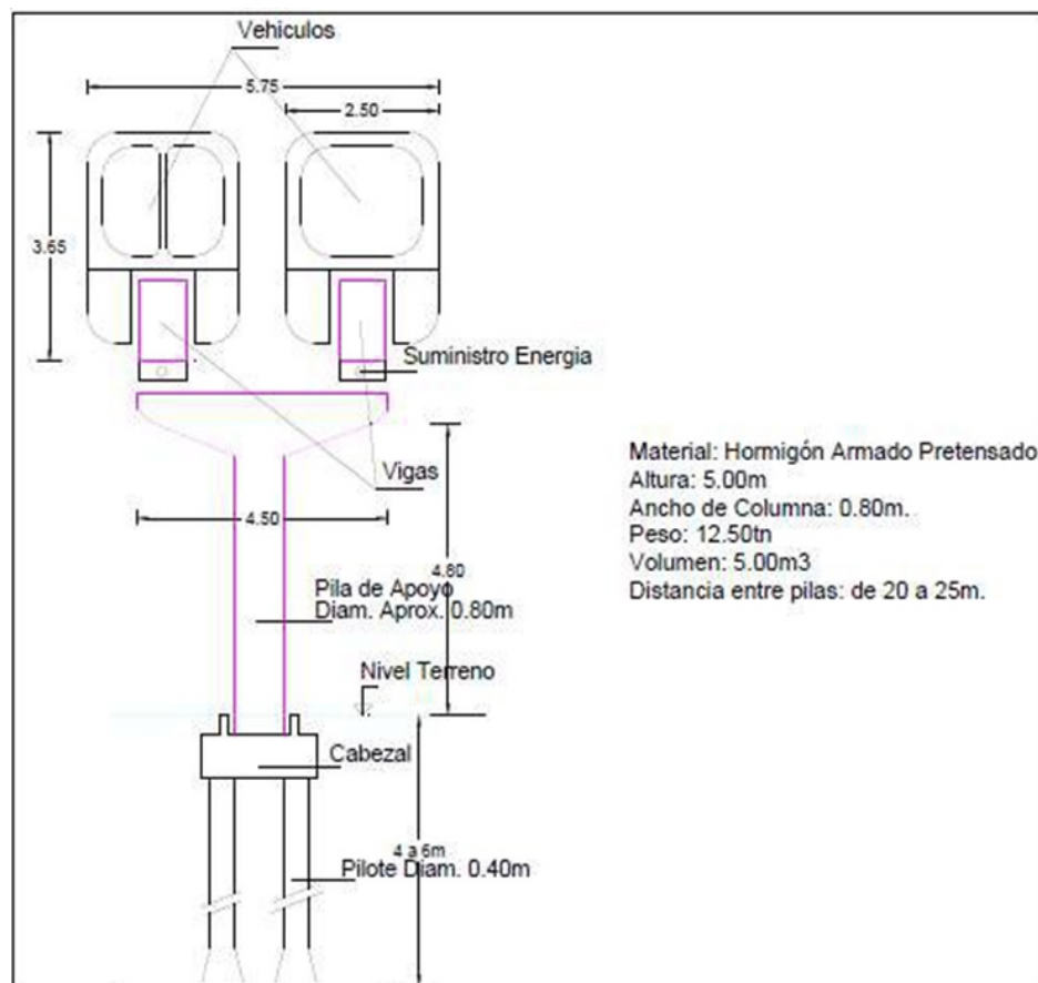
Figure 5. Cross-section of support structure
