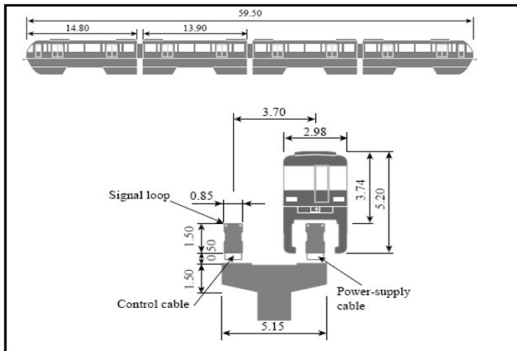
Figure 2. Four-car unit and support structure
