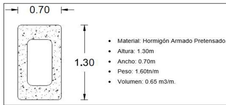
Figure 4. Cross-section of beam
