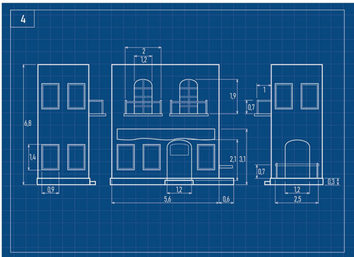
Figure 8. Blueprint
