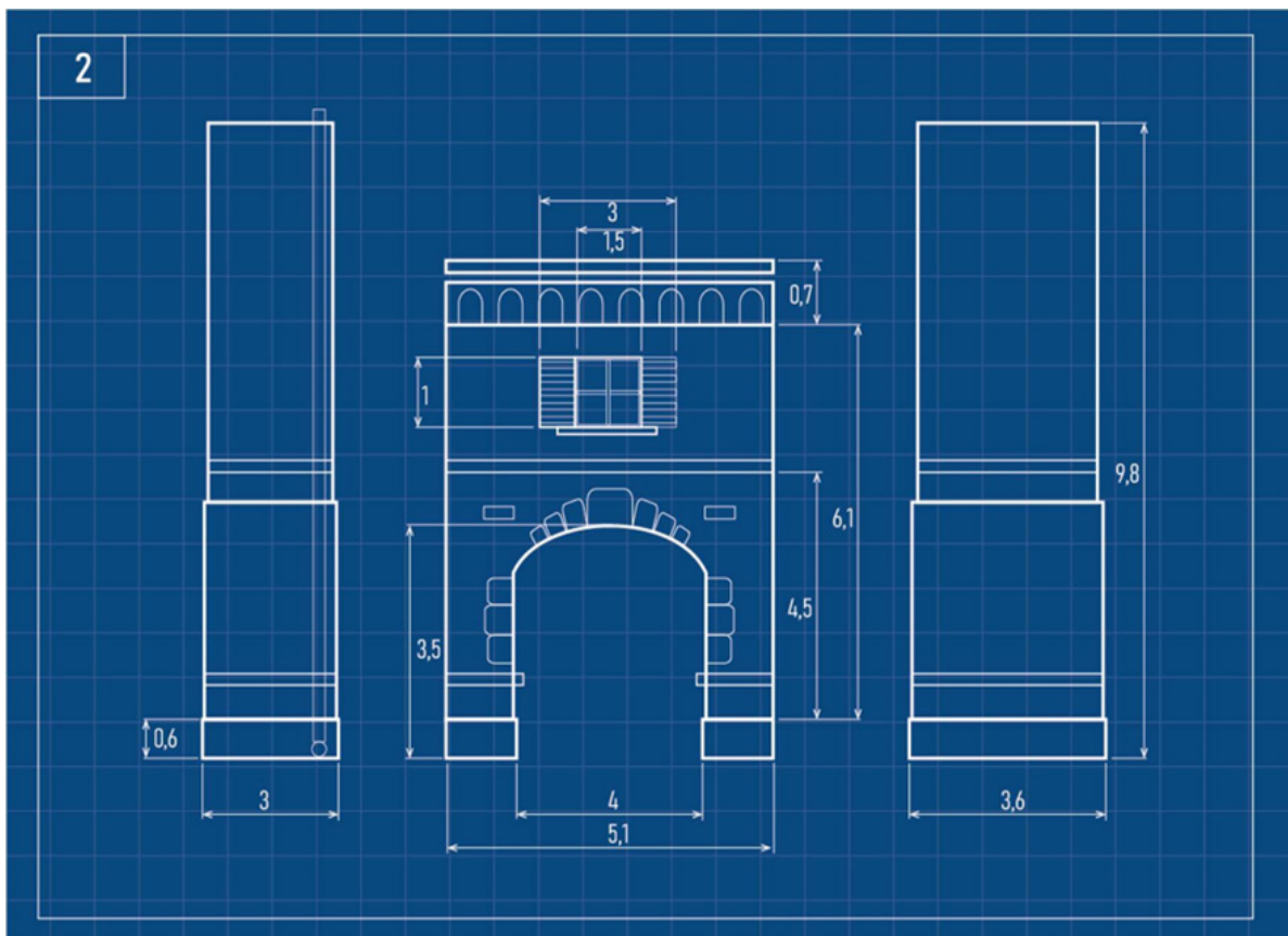
Figure 6. Blueprint
