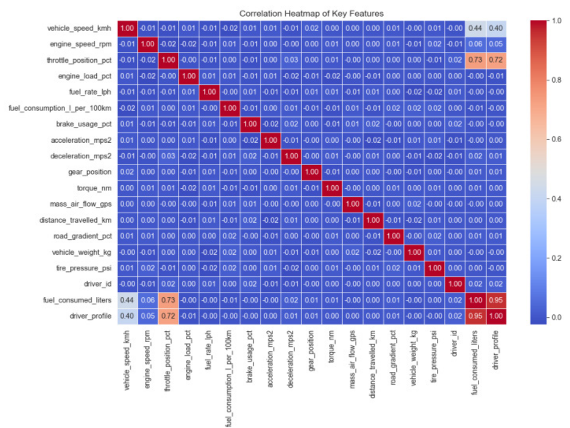
Figure 1. Correlation Heatmap of Key Features
